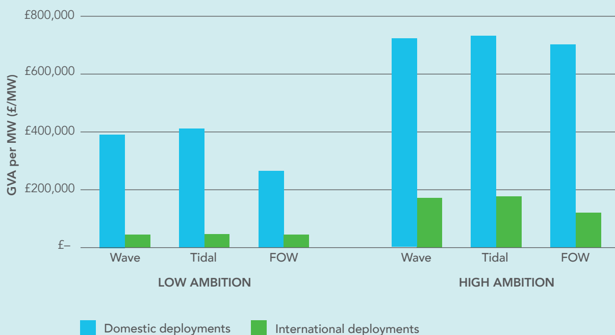
Figure 8 Breakdown of GVA per MW by technical cost centre for each scenario.
