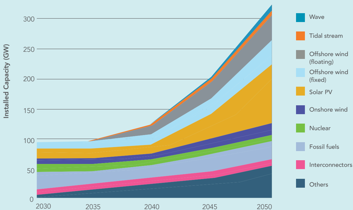
Figure 3 – UK deployed capacity from ESME modelling based on SET Plan cost targets for wave, tidal stream and floating offshore wind.
