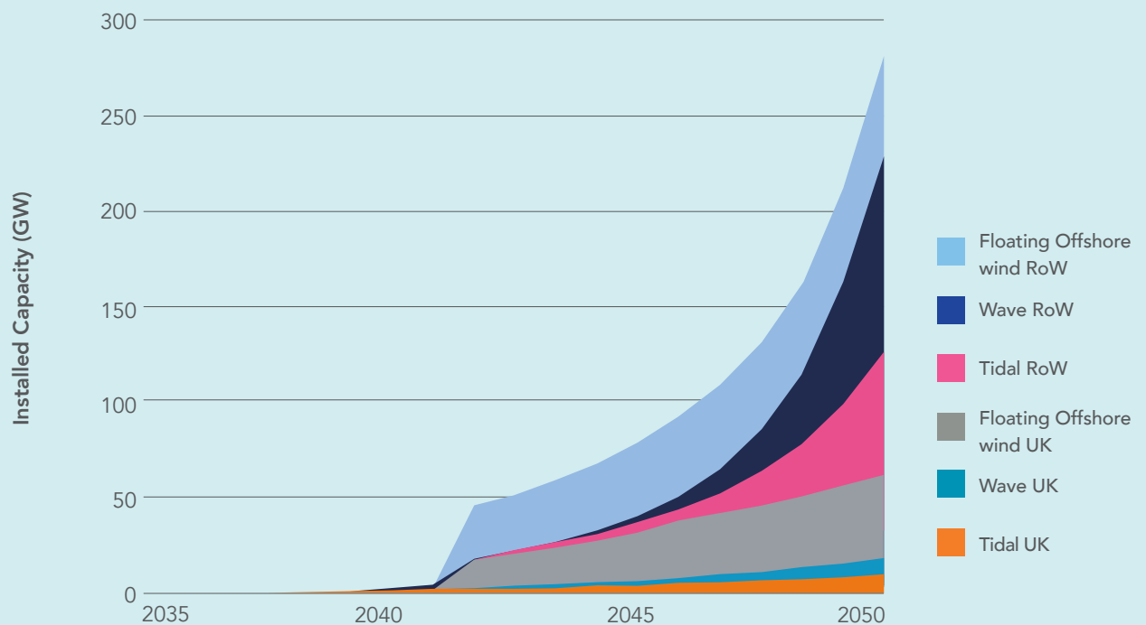
Figure 4 – Deployment trajectories for wave, tidal stream and floating offshore wind to 2050,
